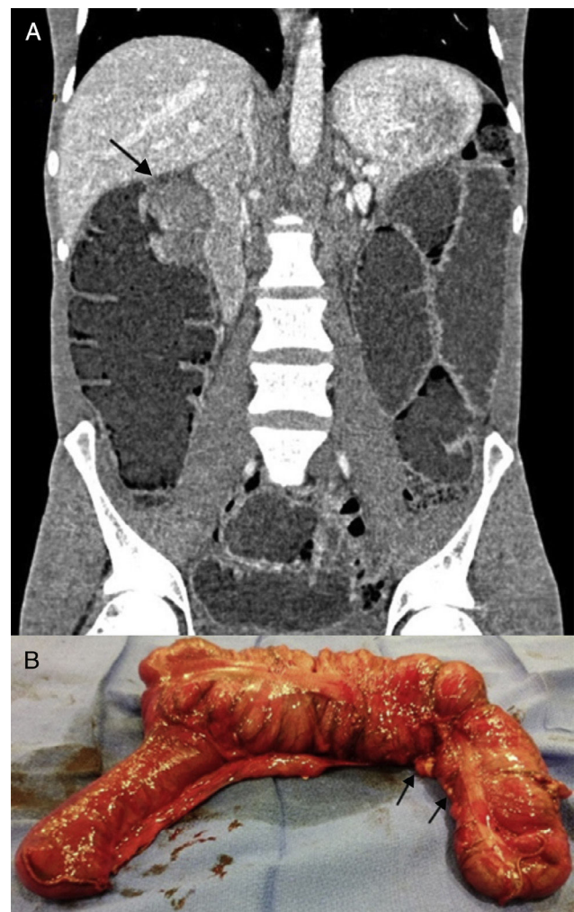
Figure 2 A) Abdominal CT scan that detected a mass at the level of the hepatic angle, suggesting an obstructive cause. B) Macroscopic study of the surgical specimen (right colon) with multiple implants (arrows) suggestive of diffuse carcinomatosis.
