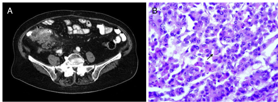
Figure 1 A) Abdominal CT scan showing irregular thickening of the cecum, with pericecal fat and terminal ileum infiltration, as well as multiple regional adenopathies. B) Histology study (H/E stain, x400): adenocarcinoma of the colon with signet ring cell pattern (arrow).
